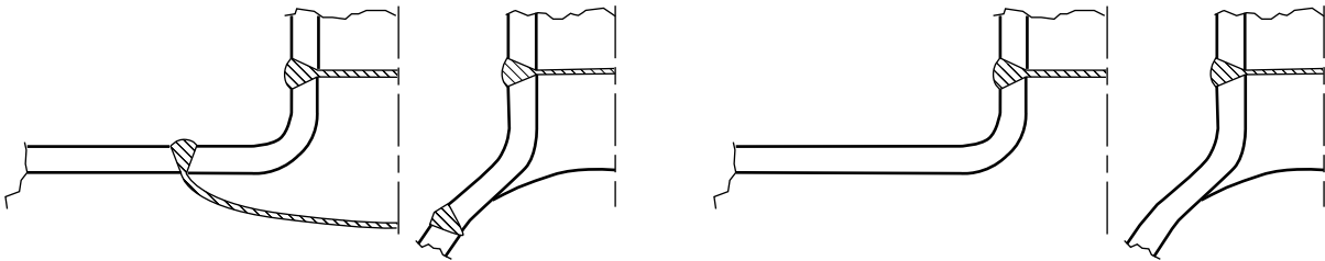
Figure GR-3.4.9-4 Acceptable Details for Branch Attachment Suitable for 100% Radiography
