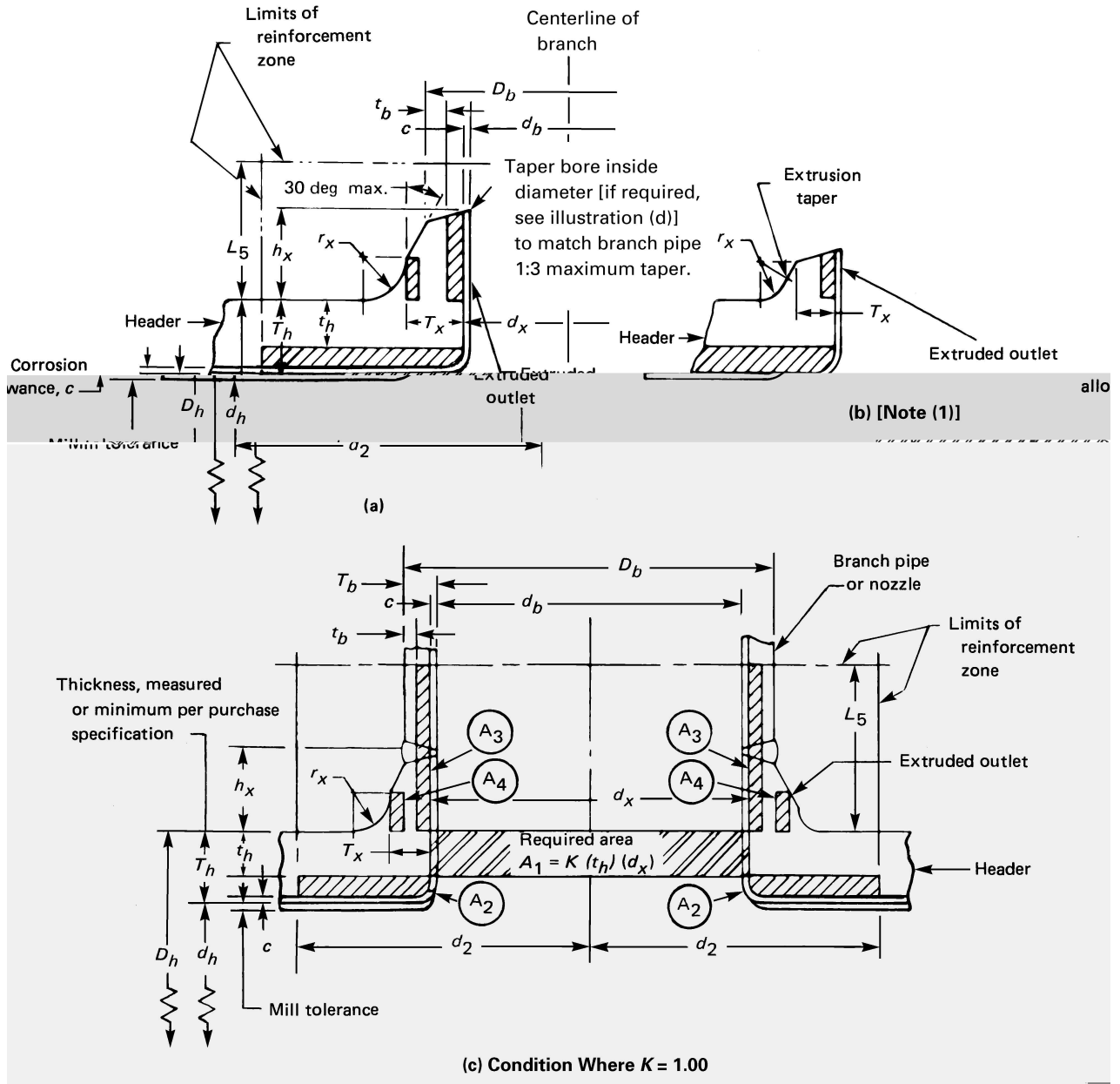
Figure IP-3.4.3-1 Extruded Outlet Header Nomenclature
