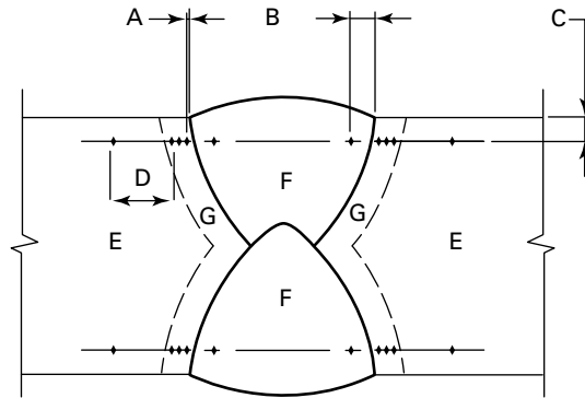
Figure GR-3.10-1 Location of Vickers Hardness Indentations
