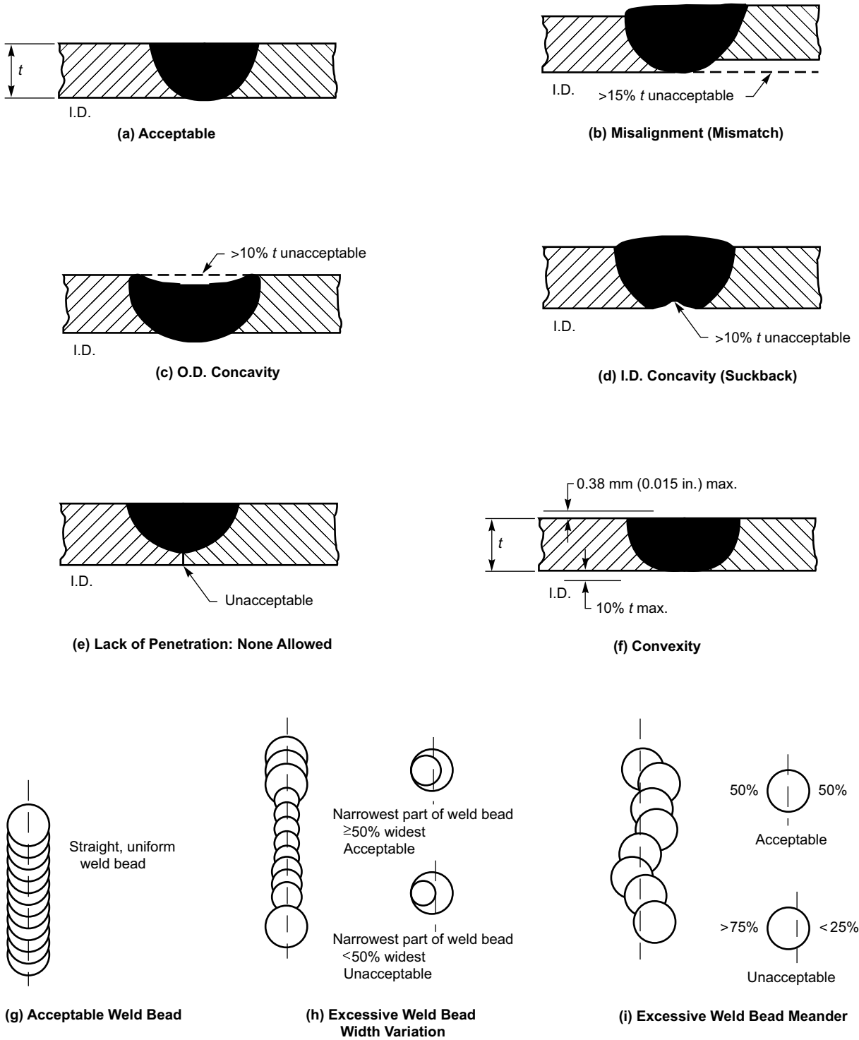
Figure A-3.5-1 Weld Quality Illustrations for Autogenous Welded Pipe or Tube
