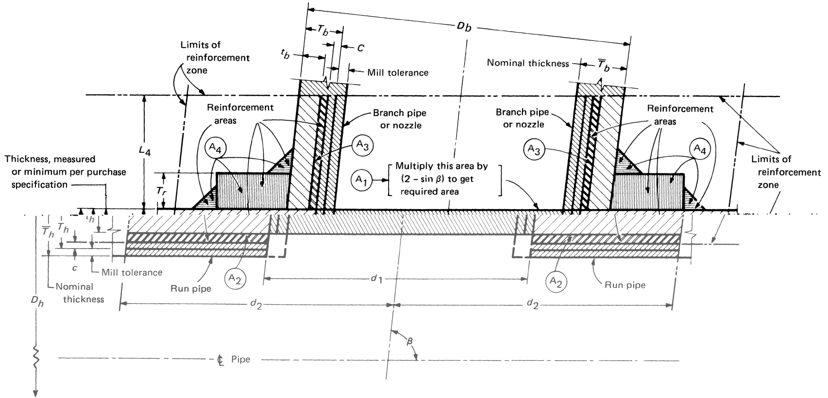
Figure IP-3.4.2-1 Branch Connection Nomenclature
