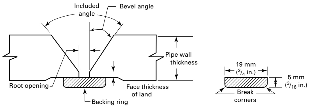
Figure GR-3.4.3-6 Geometry of Weld Joint Detail Single Vee Groove Butt, Continuous Flat Backing Ring
