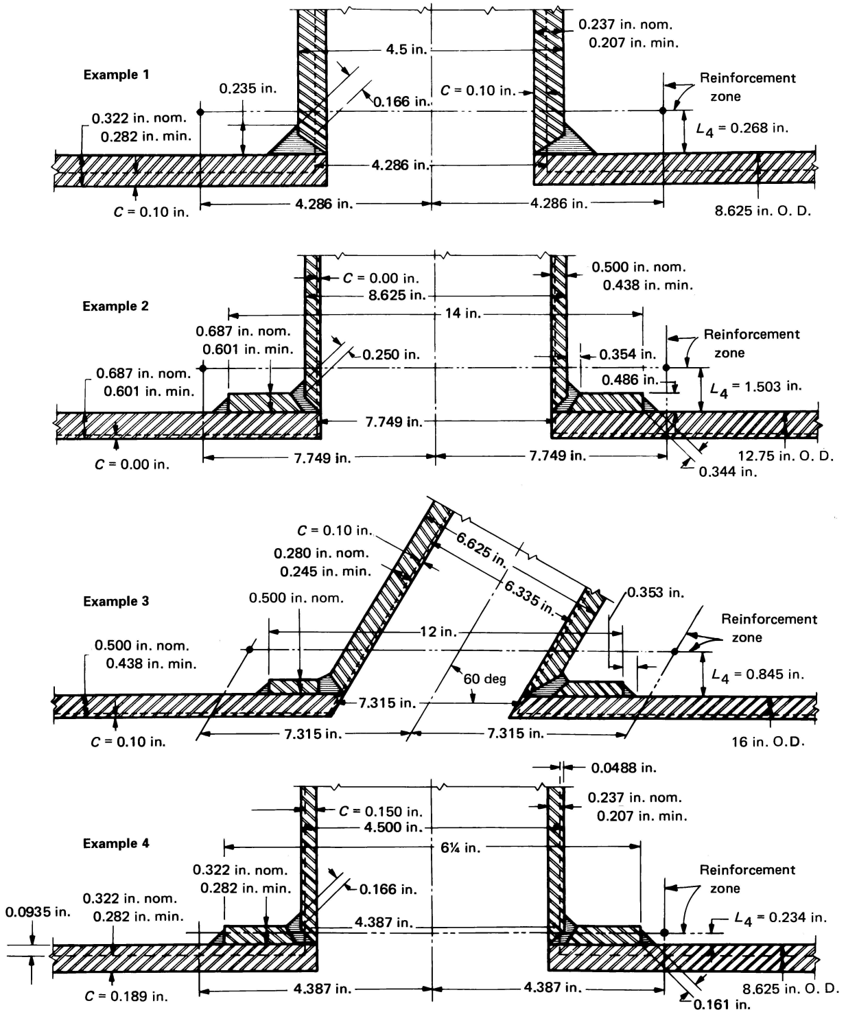
Figure E-2-1 Illustrations for Examples in Nonmandatory Appendix E
